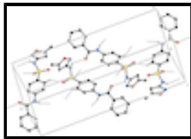
Fig. 2. A partial view of the packing of (I), showing the N—H \cdots O and C—H \cdots O hydrogen-bonding interactions (dashed lines) between the molecules. Hydrogen atoms not involved in hydrogen bonding have been omitted for clarity.
