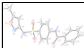
Fig. 1. View of (I) with displacement ellipsoids for non-H atoms drawn at the 30% probability level.
